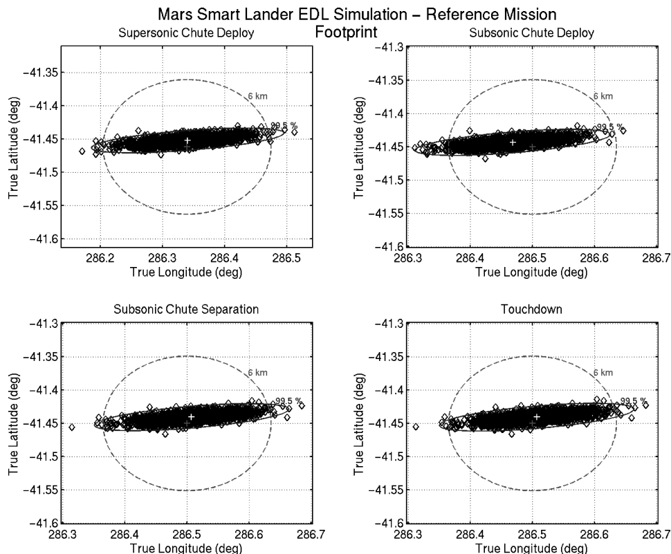
Fig. 6 Sample Monte Carlo results of footprints throughout EDL (trim shelf configuration).
