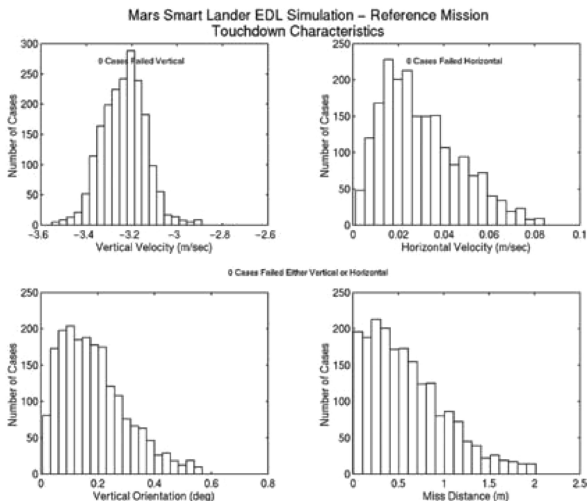
Fig. 7 Sample Monte Carlo results at touchdown (trim shelf configuration).
